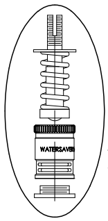
TIN-LINED SELF-CLOSING WATER SAVER RENEWABLE UNIT WITH REPLACEABLE STAINLESS STEEL SEAT
